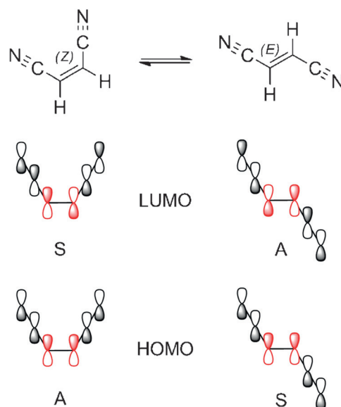
Figure 2. The cis-trans isomerization reaction between maleonitrile (left) and fumaronitrile (right). The HOMO and LUMO orbitals of the reactant and the product are also depicted along with their symmetry with respect to the C_2 symmetry axis of each molecule. S or A indicates symmetric or antisymmetric with respect to the C_2 rotation.
